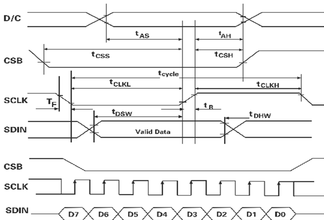
Figure 10-4-4: Serial interface characteristics
